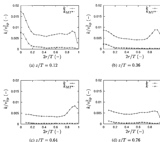
Figure 12. Radial profiles of the kinetic energy at several axial positions (Case IV). A distinction between kinetic energy and MI kinetic energy is made.
